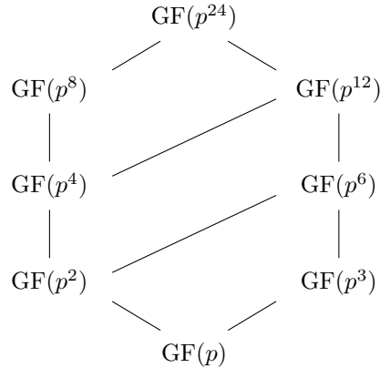
Figure 22.9: Subfields of \text{GF}(p^{24})
