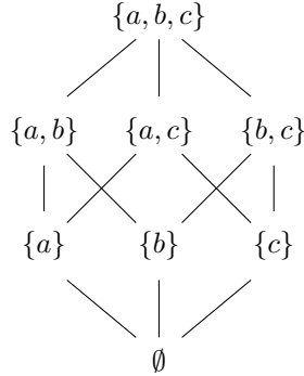
Figure 19.3: Partial order on \mathcal{P}(\{a, b, c\})
