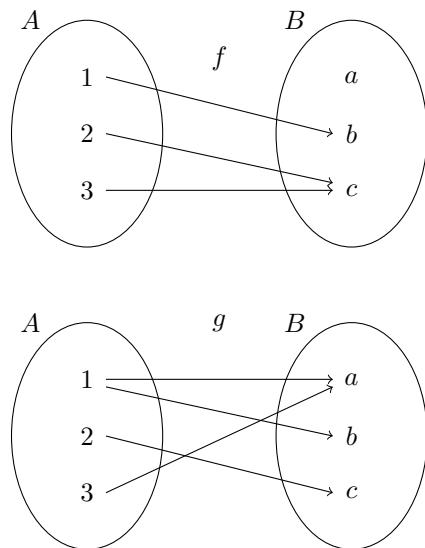
Figure 1.6: Mappings and relations
