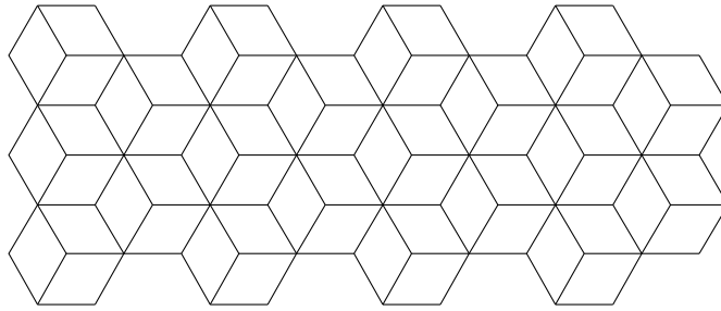
Figure 12.26
