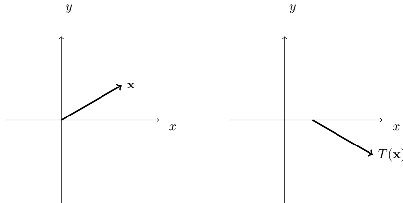
Figure 12.12: Glide reflections
