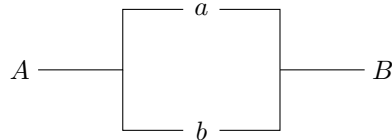
Figure 19.26: a \vee b
