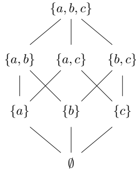
Figure 19.3: Partial order on \mathcal{P}(\{a, b, c\})
