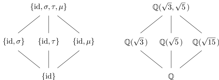
Figure 23.21: G(\mathbb{Q}(\sqrt{3}, \sqrt{5})/\mathbb{Q})
